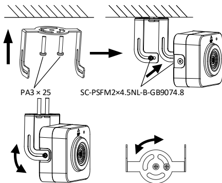
Figure 2-1 Ceiling Mounting
