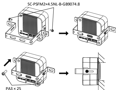
Figure 2-2 Wall Mounting
